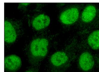
LOC728628 (C-12): sc-85698. Immunofluorescence staining of formalin-fixed Hep G2 cells showing nuclear localization.
