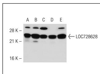
LOC728628 (C-12): sc-85698. Western blot analysis of LOC728628 expression in HeLa (A), SK-N-MC (B), NTERA-2 cl.D1 (C), Hep G2 (D) and MES-SA/Dx5 (E) whole cell lysates.
