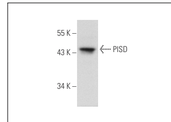
PISD (E-15): sc-86197. Western blot analysis of PISD expression in K-562 whole cell lysate.
