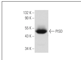
PISD (E-15): sc-86197. Western blot analysis of PISD expression in JAR whole cell lysate.
