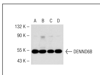
DENND6B (S-18): sc-86444. Western blot analysis of DENND6B expression in HeLa (A), U-698-M (B), SW-13 (C) and Ramos (D) whole cell lysates.
