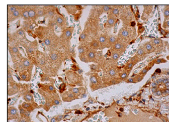
MLC1 (C-18): sc-86740. Immunoperoxidase staining of formalin fixed, paraffin-embedded human liver tissue showing cytoplasmic staining of hepatocytes, bile duct cells and hepatic sinusoids.
