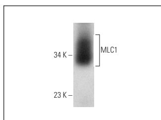
MLC1 (C-18): sc-86740. Western blot analysis of MLC1 expression in human hippocampus tissue extract.
