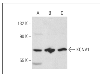
KCNV1 (P-14): sc-87181. Western blot analysis of KCNV1 expression in U-87 MG (A), IMR-32 (B) and TE671 (C) whole cell lysates.
