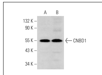
CNBD1 (N-18): sc-87641. Western blot analysis of CNBD1 expression in NTERA-2 cl.D1 (A) and HeLa (B) whole cell lysates.
