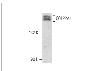
COL22A1 (N-17): sc-87647. Western blot analysis of COL22A1 expression in A-10 whole cell lysate.
