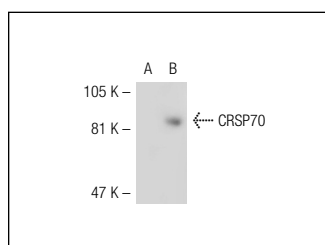
CRSP70 (C-19): sc-9425. Western blot analysis of CRSP70 expression in non-transfected: sc-117752 (A) and human CRSP70 transfected: sc-112474 (B) 293T whole cell lysates.
