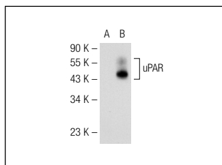
uPAR (N-19): sc-9793. Western blot analysis of uPAR expression in non-transfected: sc-117752 (A) and human uPAR transfected: sc-170817 (B) 293T whole cell lysates.
