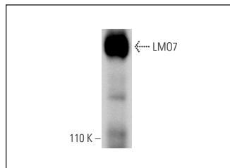
LMO7 (H-300): sc-98423. Western blot analysis of LMO7 expression in HeLa whole cell lysate.
