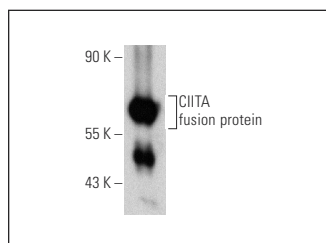
CIITA (V-19): sc-9869. Western blot analysis of human recombinant CIITA fusion protein.
