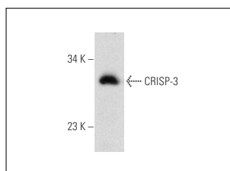
CRISP-3 (M-79): sc-98745. Western blot analysis of CRISP-3 expression in mouse embryo tissue extract.
