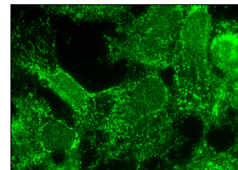
E3BP (H-130): sc-98752. Immunofluorescence staining of formalin-fixed Hep G2 cells showing mitochondria localization.
