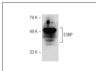
E3BP (H-130): sc-98752. Western blot analysis of E3BP expression in Hep G2 whole cell lysate.
