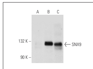
SNX9 (H-46): sc-99027. Western blot analysis of SNX9 expression in non-transfected 293T: sc-117752 (A), human SNX9 transfected 293T: sc-174107 (B) and 3T3-L1 (C) whole cell lysates.
