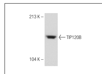
TIP120B (N-14): sc-99664. Western blot analysis of TIP120B expression in Jurkat nuclear extract.
