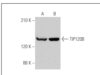
TIP120B (N-14): sc-99664. Western blot analysis of TIP120B expression in C2C12 (A) and HEK293 (B) whole cell lysates.
