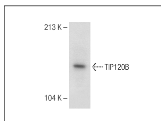
TIP120B (T-17): sc-99666. Western blot analysis of TIP120B expression in Jurkat nuclear extract.
