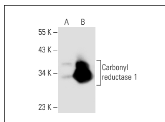
Carbonyl reductase 1 (Z-8): sc-100518. Western blot analysis of Carbonyl reductase 1 expression in non-transfected: sc-117752 (A) and mouse Carbonyl reductase 1 transfected: sc-118997 (B) 293T whole cell lysates.
