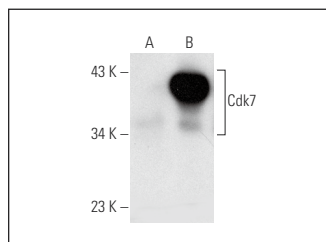
Cdk7 (D-5): sc-271794. Western blot analysis of Cdk7 expression in non-transfected: sc-110760 (A) and human Cdk7 transfected: sc-110468 (B) 293 whole cell lysates.
