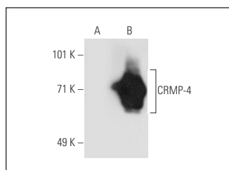
CRMP-4 (LL-5): sc-100323. Western blot analysis of CRMP-4 expression in non-transfected: sc-117752 (A) and human CRMP-4 transfected: sc-111426 (B) 293T whole cell lysates.
