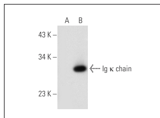
Ig \kappa chain (L1C1): sc-59265. Western blot analysis of Ig \kappa chain expression in non-transfected: sc-117752 (A) and human Ig \kappa chain transfected: sc-111799 (B) 293T whole cell lysates.
