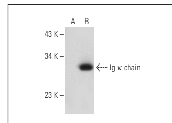
Ig \kappa chain (KP-53): sc-59264. Western blot analysis of Ig \kappa chain expression in non-transfected: sc-117752 (A) and human Ig \kappa chain transfected: sc-111799 (B) 293T whole cell lysates.
