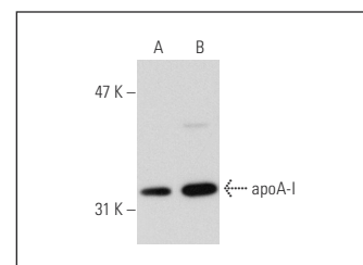
apoA-I (12C8): sc-80551. Western blot analysis of apoA-I expression in non-transfected: sc-117752 (A) and human apoA-I transfected: sc-111827 (B) 293T whole cell lysates.
