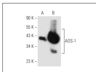
AOS-1 (H-7): sc-271592. Western blot analysis of AOS-1 expression in non-transfected: sc-110760 (A) and human AOS-1 transfected: sc-112313 (B) 293 whole cell lysates.
