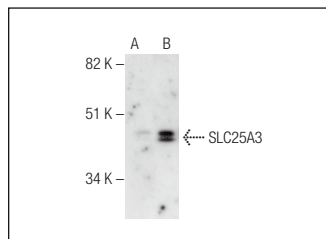
SLC25A3 (F-1): sc-376742. Western blot analysis of SLC25A3 expression in non-transfected: sc-117752 (A) and human SLC25A3 transfected: sc-113441 (B) 293T whole cell lysates.
