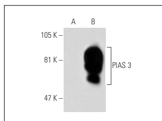
PIAS 3 (C-12): sc-46682. Western blot analysis of PIAS 3 expression in non-transfected: sc-117752 (A) and human PIAS 3 transfected: sc-114958 (B) 293T whole cell lysates.
