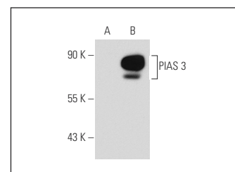
PIAS 3 (E-3): sc-48339. Western blot analysis of PIAS 3 expression in non-transfected: sc-117752 (A) and human PIAS 3 transfected: sc-114958 (B) 293T whole cell lysates.
