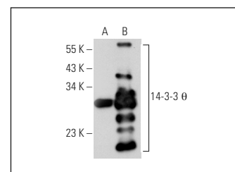
14-3-3 \theta (5J20): sc-69720. Western blot analysis of 14-3-3 \theta expression in non-transfected: sc-117752 (A) and human 14-3-3 \theta transfected: sc-116633 (B) 293T whole cell lysates.
