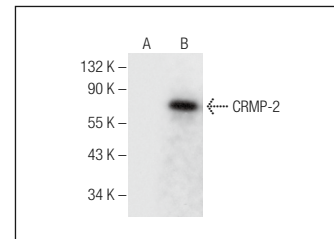
CRMP (D-5): sc-377155. Western blot analysis of CRMP-2 expression in non-transfected: sc-117752 (A) and human CRMP-2 transfected: sc-116652 (B) 293T whole cell lysates.
