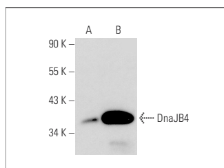
DnaJB4 (R-07): sc-100711. Western blot analysis of DnaJB4 expression in non-transfected: sc-117752 (A) and mouse DnaJB4 transfected: sc-119798 (B) 293T whole cell lysates.
