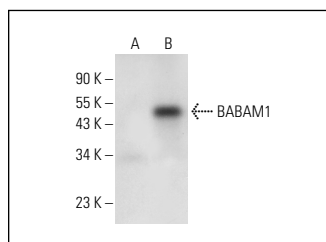
BABAM1 (H-10): sc-398570. Western blot analysis of BABAM1 expression in non-transfected: sc-117752 (A) and human BABAM1 transfected: sc-128160 (B) 293T whole cell lysates.
