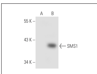
SMS1 (G-8): sc-133135. Western blot analysis of SMS1 expression in non-transfected: sc-117752 (A) and human SMS1 transfected: sc-115592 (B) 293T whole cell lysates.
