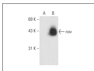
nov (F-11): sc-136965. Western blot analysis of nov expression in non-transfected: sc-117752 (A) and human nov transfected: sc-159751 (B) 293T whole cell lysates.
