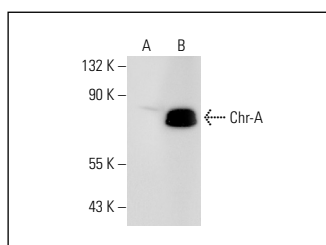
Chr-A (LK2H10): sc-47714. Western blot analysis of Chr-A expression in non-transfected: sc-117752 (A) and human Chr-A transfected: sc-159285 (B) 293T whole cell lysates
