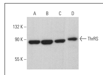
ThrRS (B-6): sc-166211. Western blot analysis of ThrRS expression in U-251-MG (A), F9 (B) and Neuro-2A (C) whole cell lysates and rat liver tissue extract (D).
