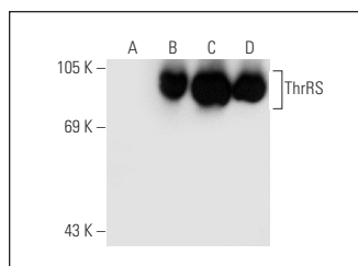
ThrRS (B-6): sc-166211. Western blot analysis of ThrRS expression in non-transfected 293T: sc-117752 (A), human ThrRS transfected 293T: sc-113560 (B), HeLa (C) and A549 (D) whole cell lysates.
