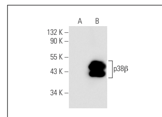
p38 \beta (BB10): sc-33689. Western blot analysis of p38 \beta expression in non-transfected: sc-117752 (A) and human p38 \beta transfected: sc-174918 (B) 293T whole cell lysates.
