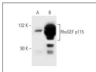
RhoGEF p115 (G-12): sc-74564. Western blot analysis of RhoGEF p115 expression in non-transfected: sc-117752 (A) and human RhoGEF p115 transfected: sc-175428 (B) 293T whole cell lysates.
