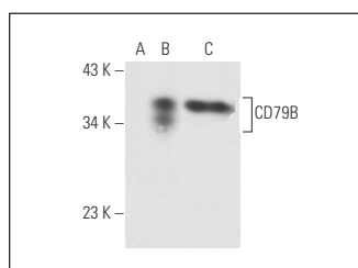
CD79B (SN8): sc-18902. Western blot analysis of CD79B expression in non-transfected 293T: sc-117752 (A), human CD79B transfected 293T: sc-115257 (B) and Raji (C) whole cell lysates.
