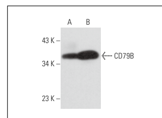
CD79B (SN8): sc-18902. Western blot analysis of CD79B expression in U-698-M (A) and Ramos (B) whole cell lysates.
