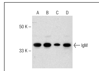
IgM (A-7): sc-373781. Western blot analysis of IgM expression in NAMALWA (A), Raji (B), U-698-M (C) and Ramos (D) whole cell lysates.
