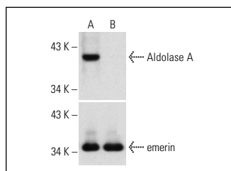
Aldolase A siRNA (h): sc-29664. Western blot analysis of Aldolase A expression in non-transfected control (A) and Aldolase A siRNA transfected (B) HeLa cells. Blot probed with Aldolase A (N-15): sc-12059. emerin (H-12): sc-25284 used as specificity and loading control.
