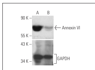
Annexin VI siRNA (h): sc-29688. Western blot analysis of Annexin VI expression in non-transfected control (A) and Annexin VI siRNA transfected (B) HeLa cells. Blot probed with Annexin VI (N-19): sc-1931. GAPDH (FL-335): sc-25778 used as specificity and loading control.
