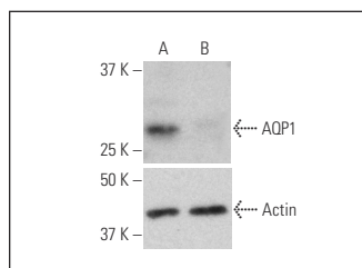
AQP1 siRNA (h): sc-29711. Western blot analysis of AQP1 expression in non-transfected control (A) and AQP1 siRNA transfected (B) HeLa cells. Blot probed with AQP1 (H-55): sc-20810. Actin (I-19): sc-1616 used as specificity and loading control.
