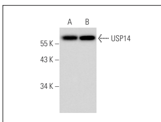
USP14 (E-17): sc-69075. Western blot analysis of USP14 expression in U-698-M (A) and Jurkat (B) whole cell lysates.
