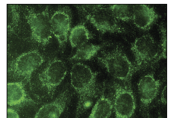
A33 (N-15): sc-33012. Immunofluorescence staining of methanol-fixed HeLa cells showing cytoplasmic localization.
