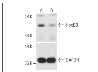
HoxD9 siRNA (h): sc-35585. Western blot analysis of HoxD9 expression in non-transfected control (A) and HoxD9 siRNA transfected (B) HeLa cells. Blot probed with HoxD9 (H-342): sc-8320. GAPDH (FL-335): sc-25778 used as specificity and loading control.
