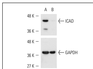
ICAD siRNA (h): sc-35624. Western blot analysis of ICAD expression in non-transfected control (A) and ICAD siRNA transfected (B) HeLa cells. Blot probed with ICAD (FL-331): sc-9066. GAPDH (FL-335): sc-25778 used as specificity and loading control.
