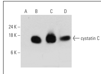
cystatin C (A-10): sc-515732. Western blot analysis of cystatin C expression in non-transfected 293T: sc-117752 (A) and human cystatin C transfected 293T: sc-117752 (B) whole cell lysates and human salivary gland (C) and human epididymis (D) tissue extracts.
