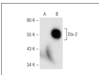
Ets-2 (G-8): sc-365584. Western blot analysis of Ets-2 expression in non-transfected: sc-117752 (A) and mouse Ets-2 transfected: sc-120131 (B) 293T whole cell lysates.
