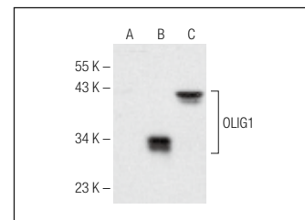
OLIG1 (H-6): sc-374294. Western blot analysis of OLIG1 expression in non-transfected 293T: sc-117752 (A), mouse OLIG1 transfected 293T: sc-122238 (B) and U-87 MG (C) whole cell lysates.
