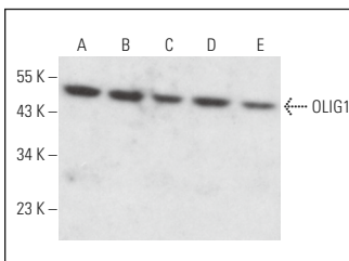
OLIG1 (H-6): sc-374294. Western blot analysis of OLIG1 expression in Daudi (A), IMR-32 (B), Neuro-2A (C), BYDP (D) and WEHI-231 (E) whole cell lysates.
