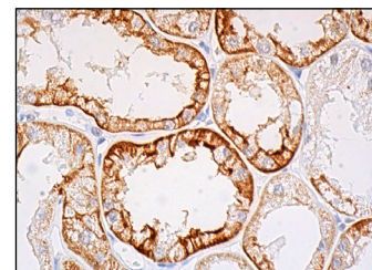
p-KV4.2 (A-5): sc-377545. Immunoperoxidase staining of formalin fixed, paraffin-embedded human kidney tissue showing membrane and cytoplasmic staining of cells in tubules.
