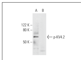
p-KV4.2 (A-5): sc-377545. Western blot analysis of KV4.2 phosphorylation in untreated (A) and lambda protein phosphatase (sc-200312A) treated (B) mouse cerebellum tissue extracts.
