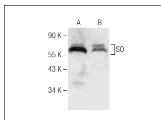
SO (G-4): sc-390322. Western blot analysis of SO expression in human liver tissue extract (A) and Hep G2 whole cell lysate (B).
