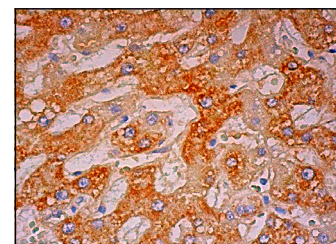
SO (G-4): sc-390322. Immunoperoxidase staining of formalin fixed, paraffin-embedded human liver tissue showing cytoplasmic staining of hepatocytes.
