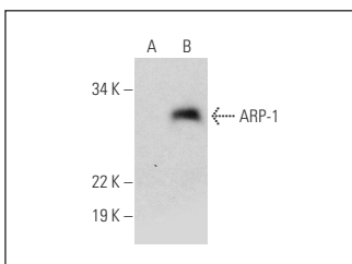
ARP-1 (C-10): sc-393481. Western blot analysis of ARP-1 expression in non-transfected: sc-117752 (A) and human ARP-1 transfected: sc-111675 (B) 293T whole cell lysates.
