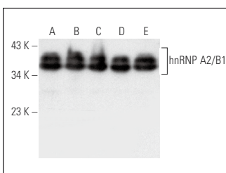
hnRNP A2/B1 (B-8): sc-393726. Western blot analysis of hnRNP A2/B1 expression in K-562 (A), THP-1 (B), Jurkat (C), HeLa (D) and MEG-01 (E) nuclear extracts.
