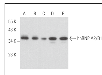
hnRNP A2/B1 (B-8): sc-393726. Western blot analysis of hnRNP A2/B1 expression in K-562 (A), HEL 92.1.7 (B), BYDP (C), WR19L (D) and c4 (E) whole cell lysates.
