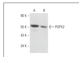
POPX2 (G-10): sc-393806. Western blot analysis of POPX2 expression in Jurkat (A) and HL-60 (B) whole cell lysates.
