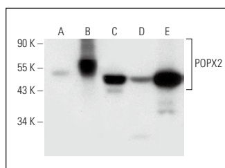
POPX2 (G-10): sc-393806. Western blot analysis of POPX2 expression in non-transfected 293T: sc-117752 (A), human POPX2 transfected 293T: sc-117752 (B), Jurkat (C), MCF7 (D) and K-562 (E) whole cell lysates.
